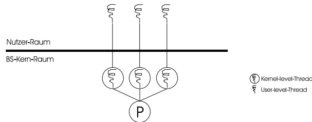
Abbildung 4.6: Kernel-level-Thread-Modell
