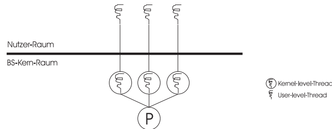
Abbildung 4.6: Kernel-level-Thread-Modell
