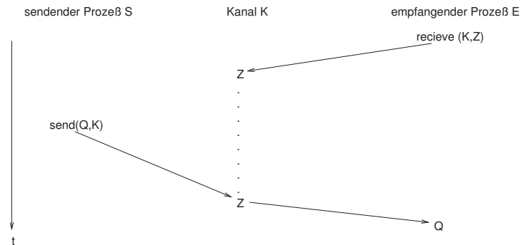
Abbildung 10.3: Receive-Send-Kommunikation (asynchron)
