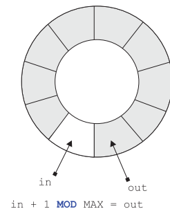
Ringpuffer – voll
