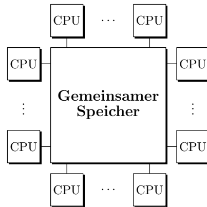
Abbildung 16.1: Shared Memory Systems
