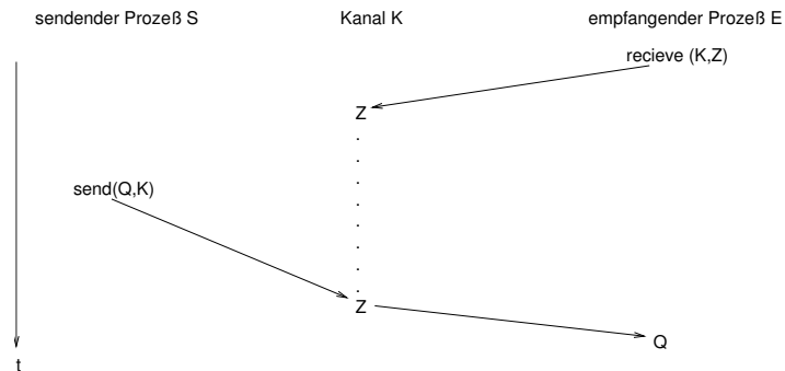
Abbildung 10.3: Receive-Send-Kommunikation (asynchron)
