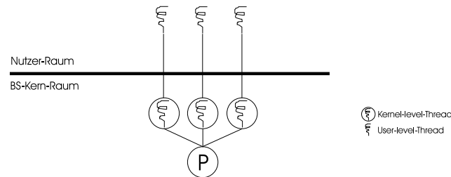
Abbildung 4.6: Kernel-level-Thread-Modell
